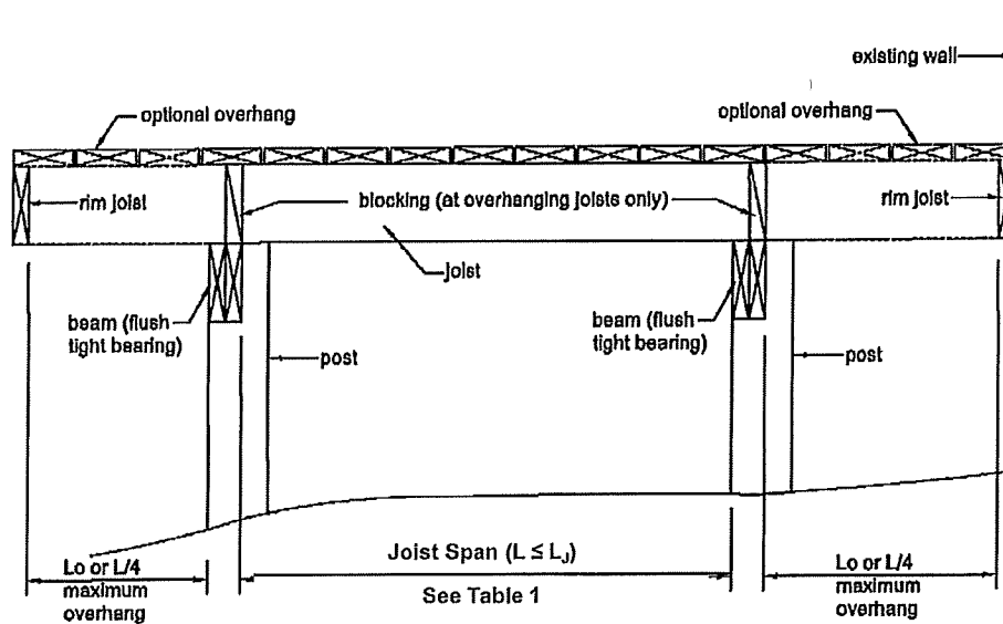
Figure 2C. Joist Span – Non-Ledger Deck
