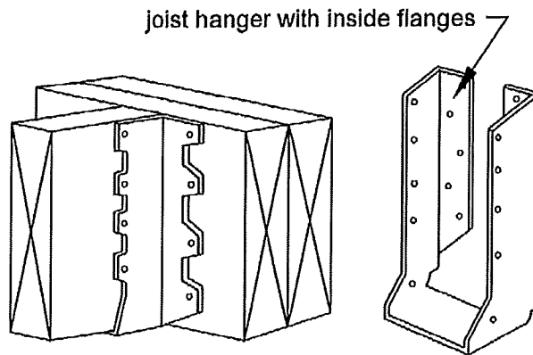
Figure 6. Typical Joist Hangers
