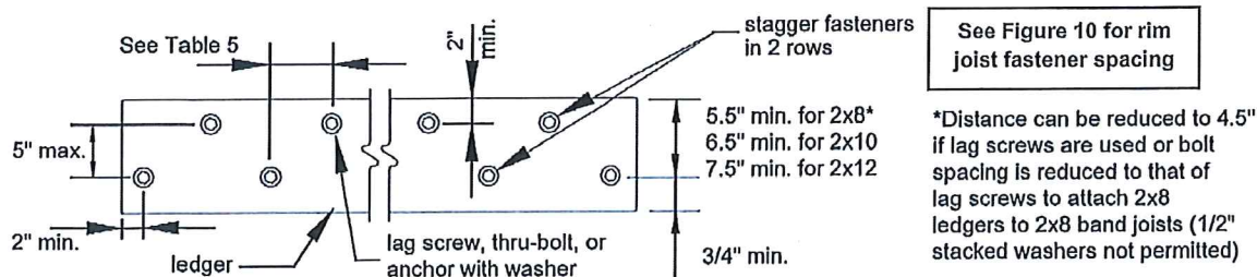
Figure 14. Ledger Fastener Spacing and Clearances
