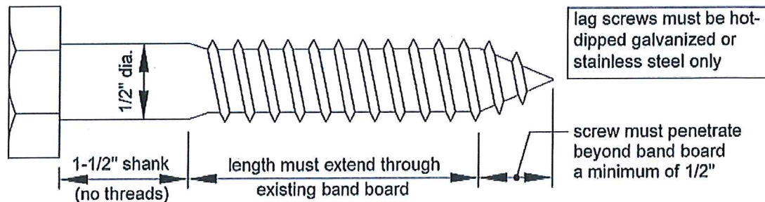
Figure 13. Lag Screw Requirements
