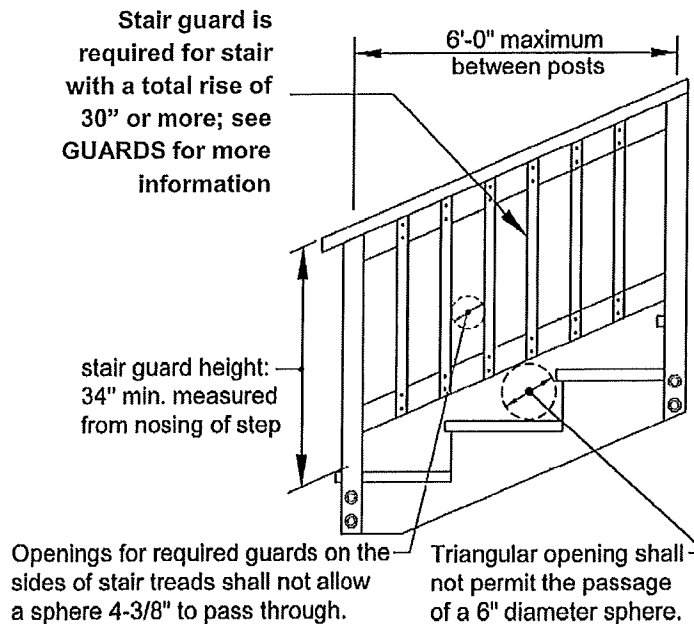
Figure 26. Stair Guard Requirements
