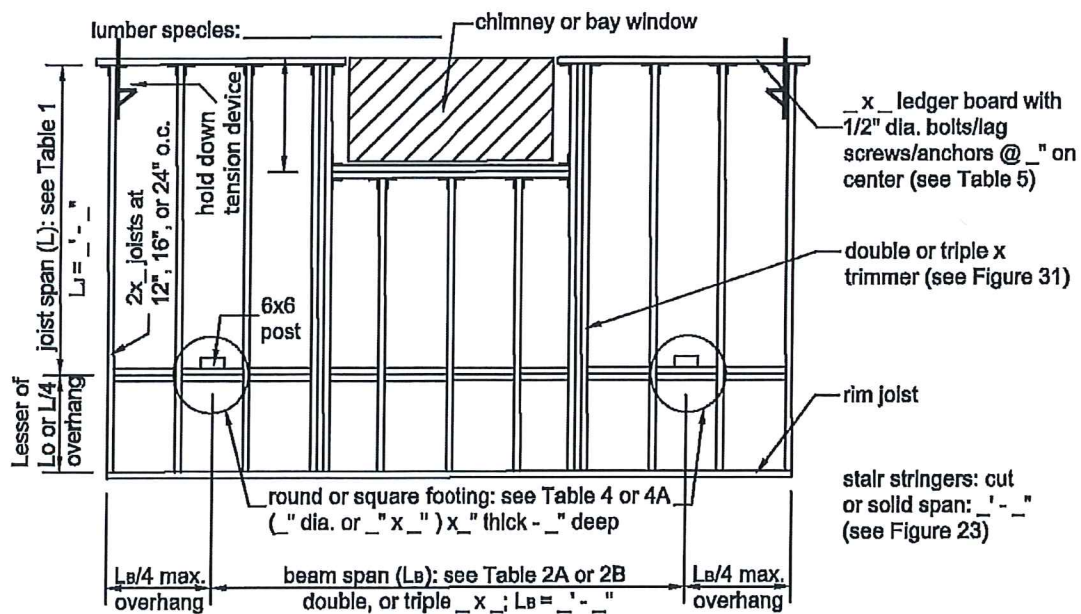
Figure 32. Typical Deck Framing Plan
