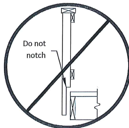
Figure 19. Post Notches Prohibited
