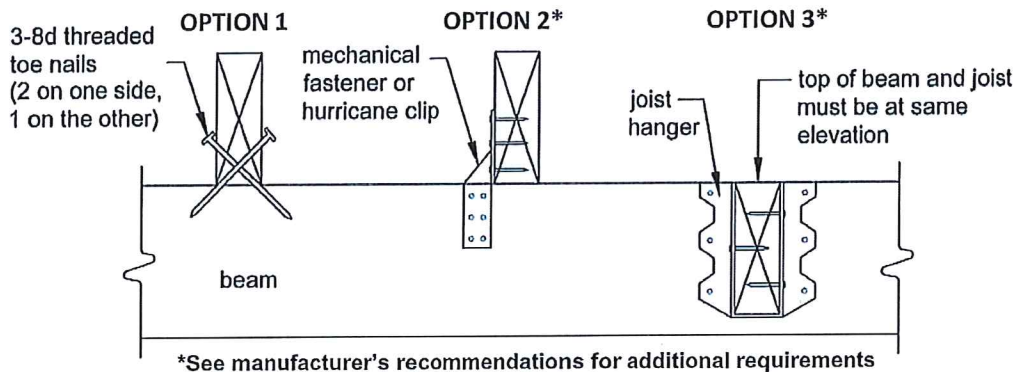
Figure 5. Joist-to-Beam Detail
