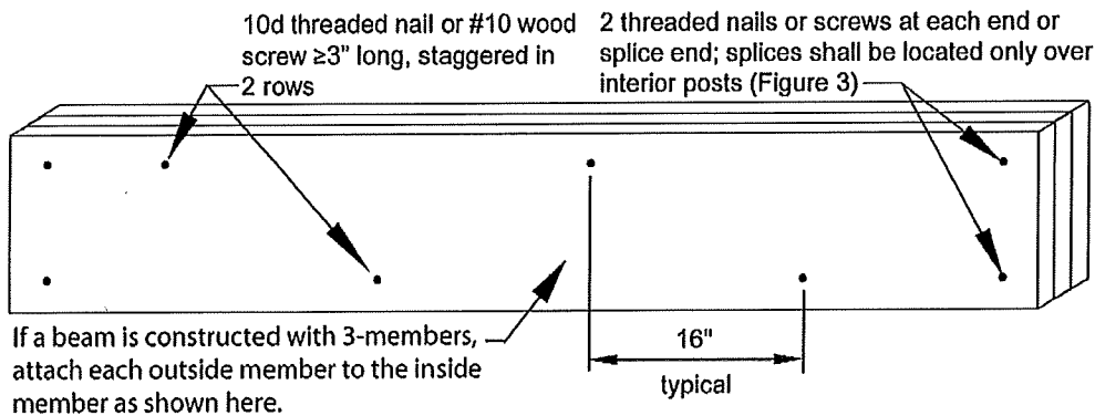
Figure 4. Beam Assembly Details
