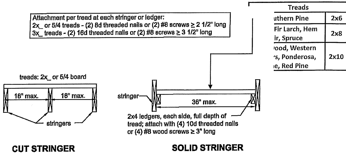
Figure 25. Tread Connection Requirements
