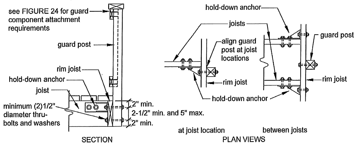
Figure 21. Guard Post to Rim Joist Example
