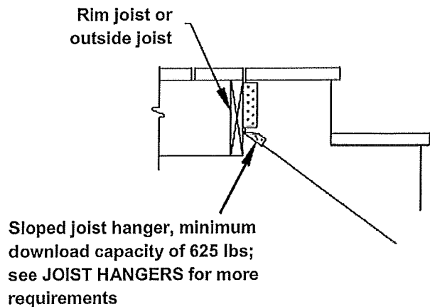
ATTACHMENT WITH HANGERS
